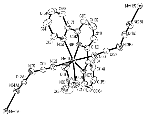
Fig. 1 An ORTEP plot (40% probability ellipsoids) and atom labelling scheme of [\text{Mn}(\mu_{1,5}\text{-dca})(\text{NO}_3)(\text{terpy})]_n 1 , with pentagonal bipyramidal \text{Mn}^{\text{II}} .
